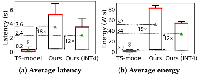
Figure 12: M4’s runtime cost of latency and energy measured on Jetson ORIN (GPU).
