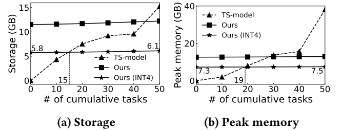
Figure 11: M4’s scalability analysis of storage and peak memory measured on Jetson ORIN.
