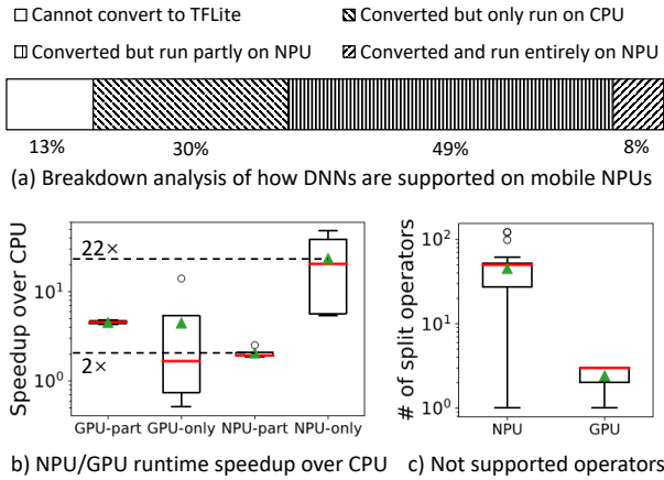
Figure 2: An empirical study of 110 in-the-wild DNNs crawled from public sources on Google Pixel 7 Pro.
