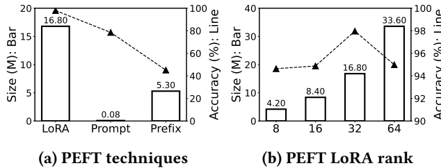
Figure 10: Impact analysis of PEFT-enhanced M4 on text classification. Size (M): trainable parameter size.
