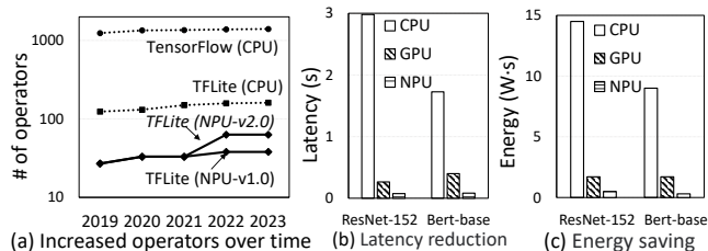
Figure 1: Empirical study on mobile NN processors: (1) A longitudinal analysis of operator support on CPU/NPU; (2) The performance gap between NPU and CPU/GPU on Google Pixel 7 Pro.
